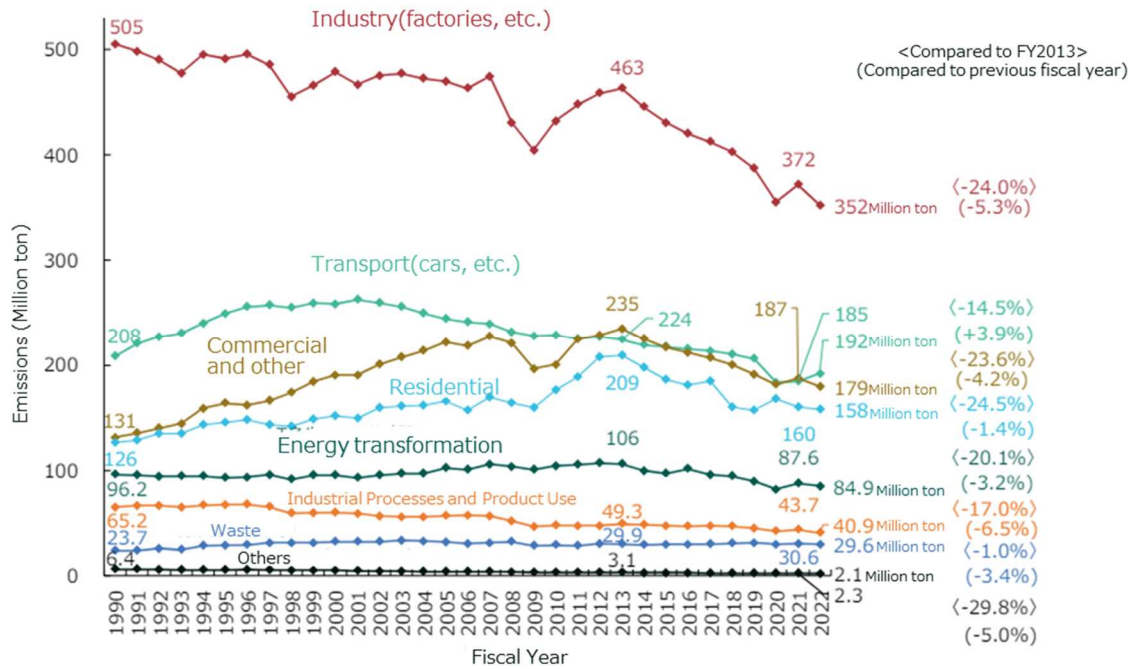
Figure 6: Trends in Japan's CO 2 Emissions by Sector 17
